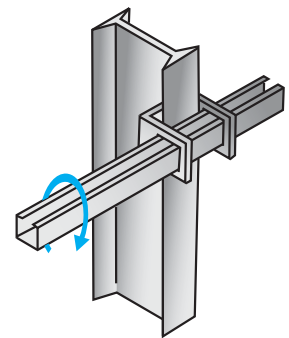
Vertical assembly
